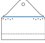
24"x20"9" bottom gusset, 1.7 mil Natural HDPE, 6" SW vents & easy open
