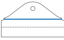
34"x19"12" bottom gusset, 2 mil Natural HDPE, 6" SW handle
