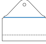
24"x20"9" bottom gusset, 1.7 mil Natural HDPE, 6" SW
